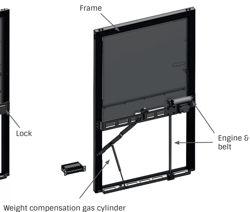
MOTORIZED VERSION
